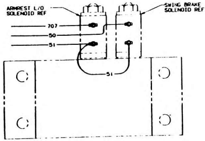
VIEW E BOTTOM VIEW ARREST L/O & SWING BRAKE SOLENOID
